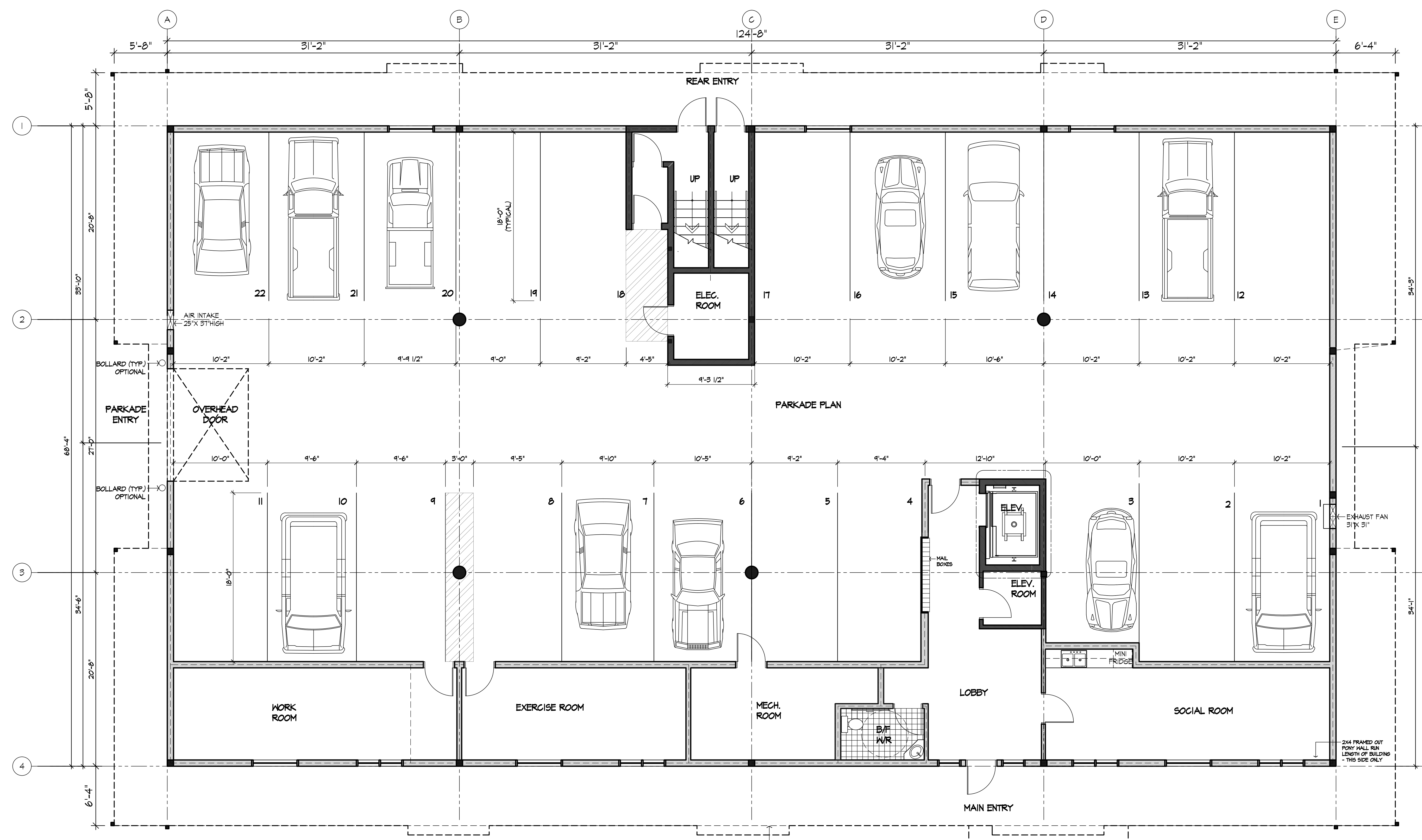
PARKADE PLAN - 22 STALLS SCALE: 3/16" = 1'-0" BUILDING AREA = 8514 SQ. FT. (791 SQ. M.)
